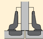
Half overlay door 9.5 mm cranking
